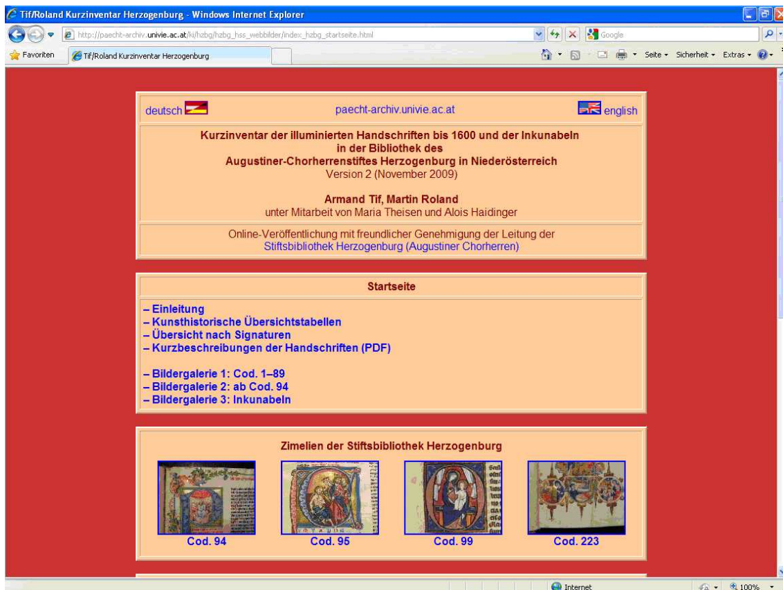
Abb. 1 – Screenshot
