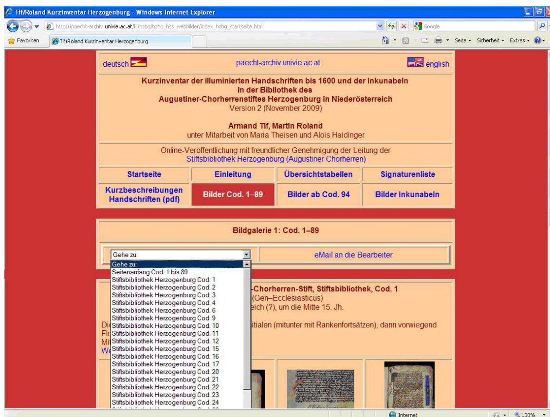
Abb. 2 – Screenshot
