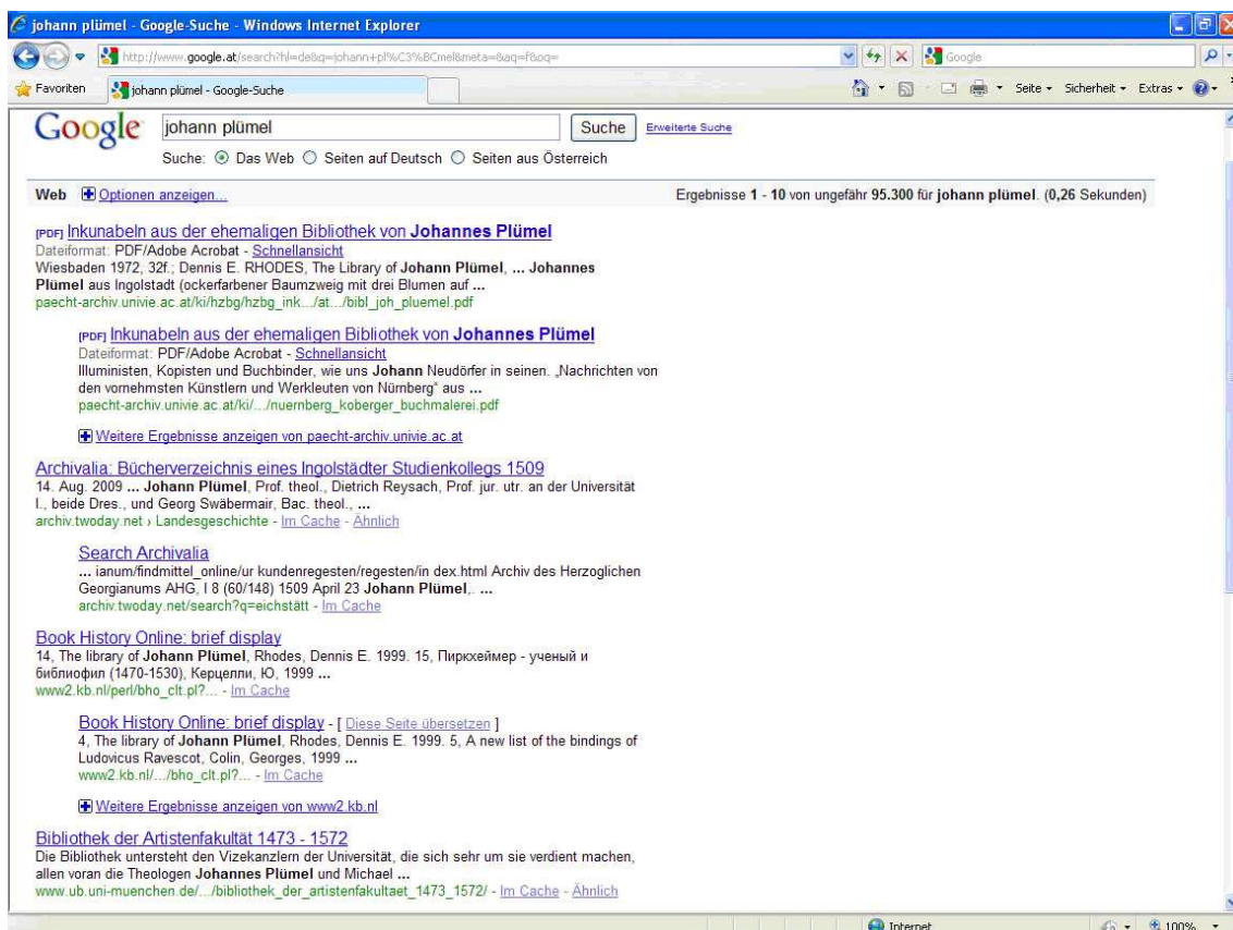
Abb. 5 – Screenshot
