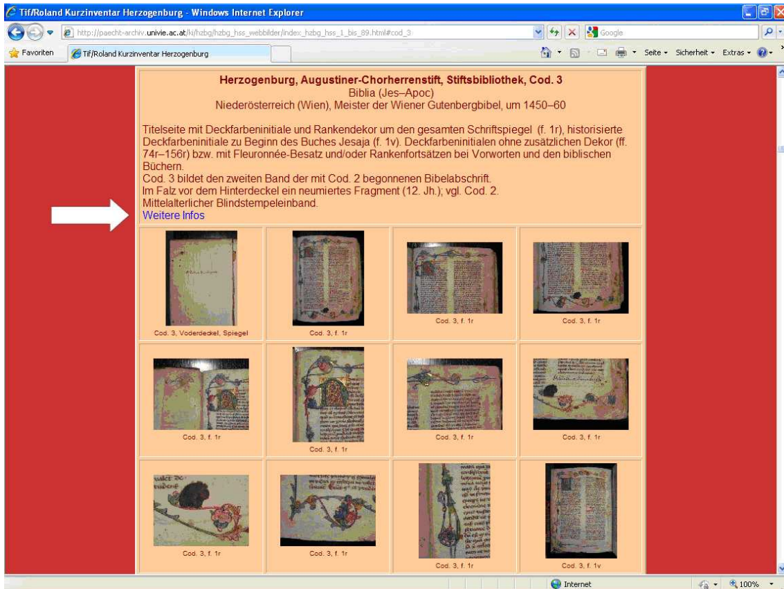
Abb. 3 – Screenshot
