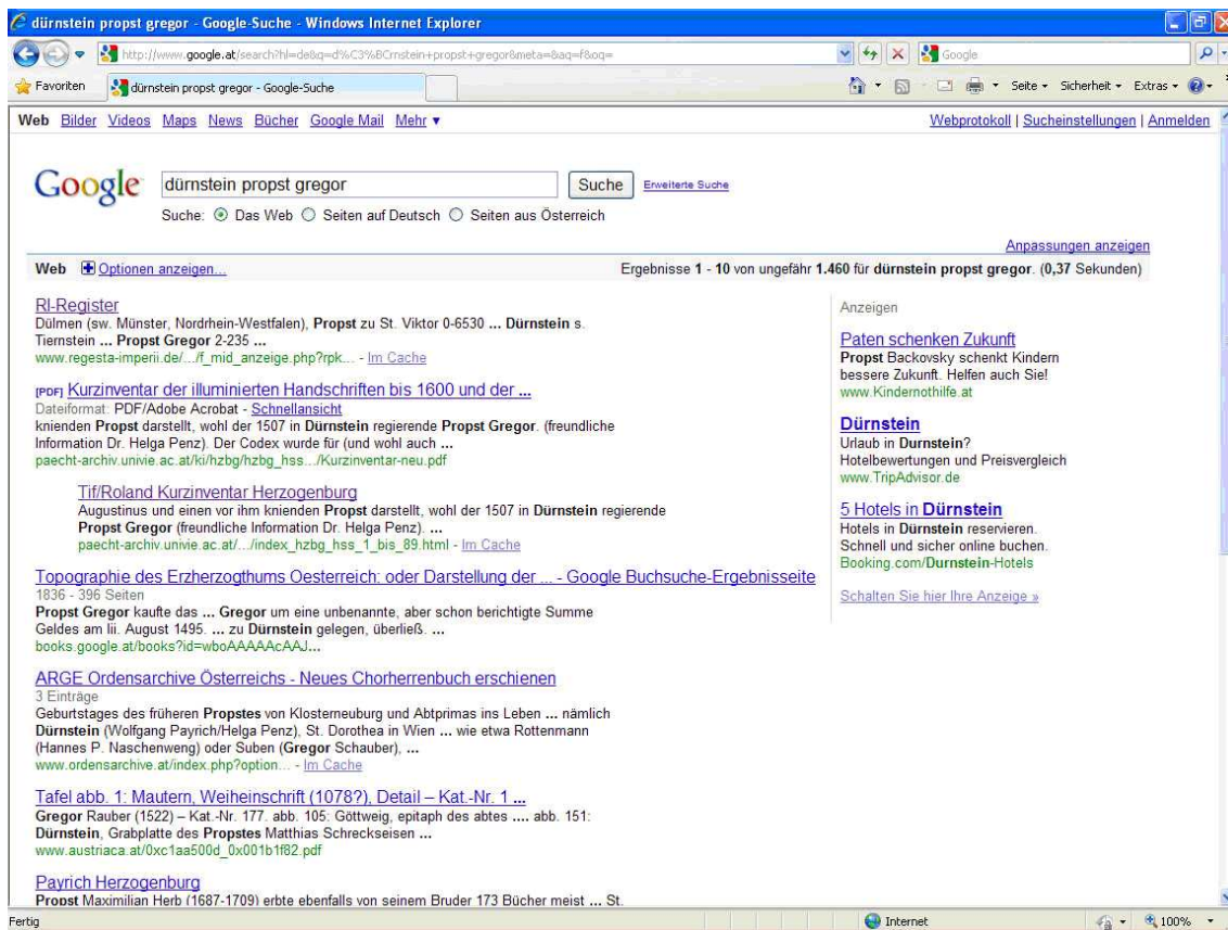
Abb. 4 – Screenshot
