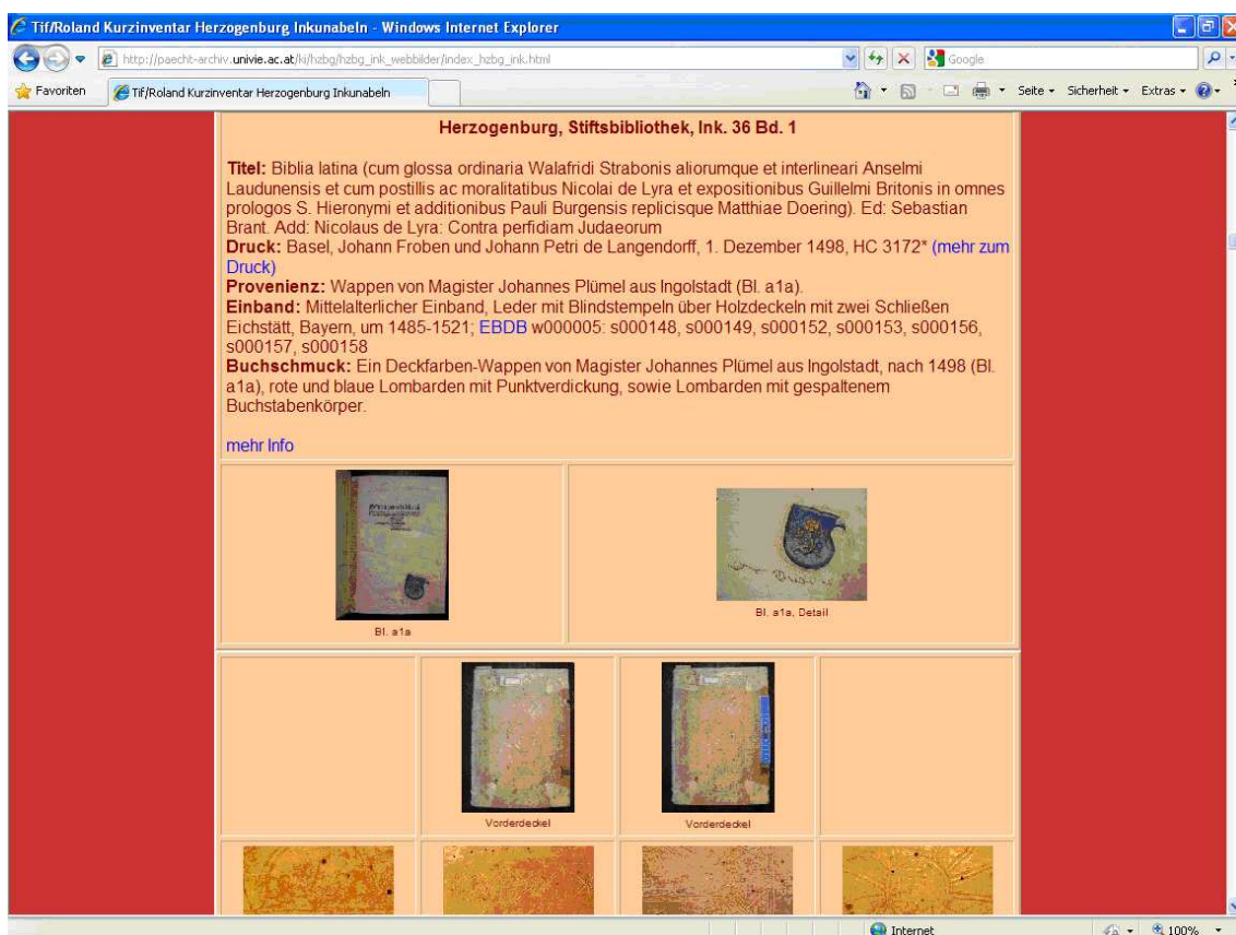
Abb. 6 – Screenshot
